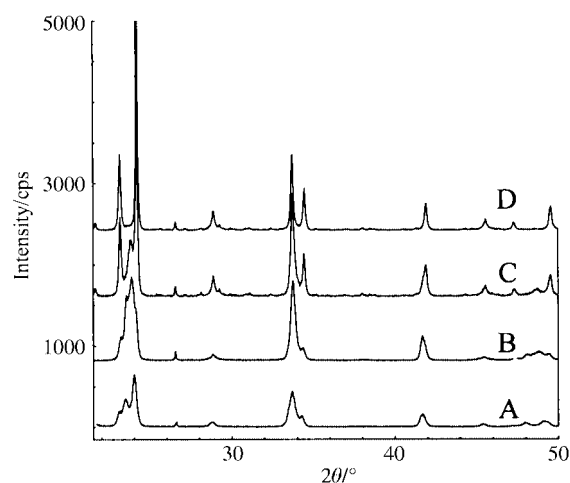
Fig. 4 The change with time of the X-ray powder diffraction patterns of a Li_{0.3}WO_3 sample. The pattern (A) was recorded during 7 hours on a wet sample covered with Parafilm. Patterns (B), (C), and (D) were recorded after the material had been exposed to air for 13, 160, and 223 hours respectively.
