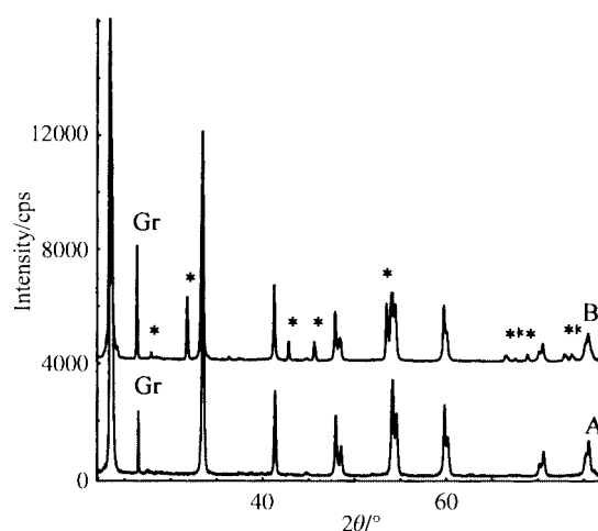
Fig. 2 X-Ray powder diffraction patterns of electrochemically prepared hydrogen intercalates of \text{WO}_3 . (A) \text{H}_{0.50}\text{WO}_3 prepared with 0.6 M nitric acid as electrolyte. (B) \text{H}_{0.50}\text{WO}_3 prepared with saturated \text{Ba}(\text{NO}_3)_2 as electrolyte solution. The intensity scales have been adjusted so that the intensities of the main peaks of the intercalates are nearly equal. Gr, reflections from graphite; *, reflections from \text{BaWO}_4 .
