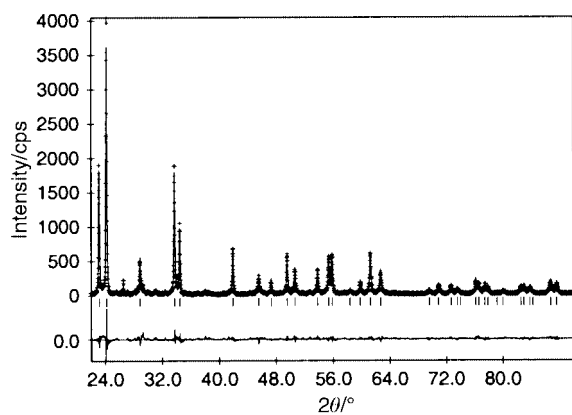
Fig. 5 Observed (crosses) and calculated (full lines) profiles for the Rietveld refinement of \text{Li}_x\text{WO}_3 . Details as in Fig. 3.
