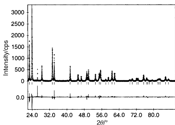
Fig. 3 Observed (crosses) and calculated (full lines) profiles for the Rietveld refinement of H_{0.12}WO_3 . The lower curve is the difference between observed and calculated profiles. A small region around 26^\circ was excluded from the refinements. At this position the strongest reflection of graphite is situated.
